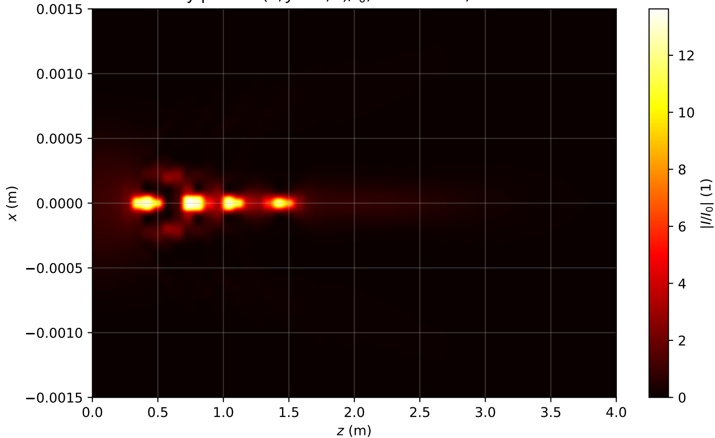
Intensity profile I(x, y = 0, z)/I_0 , \text{Pin}=8.5\text{Pcr} , artificial time
